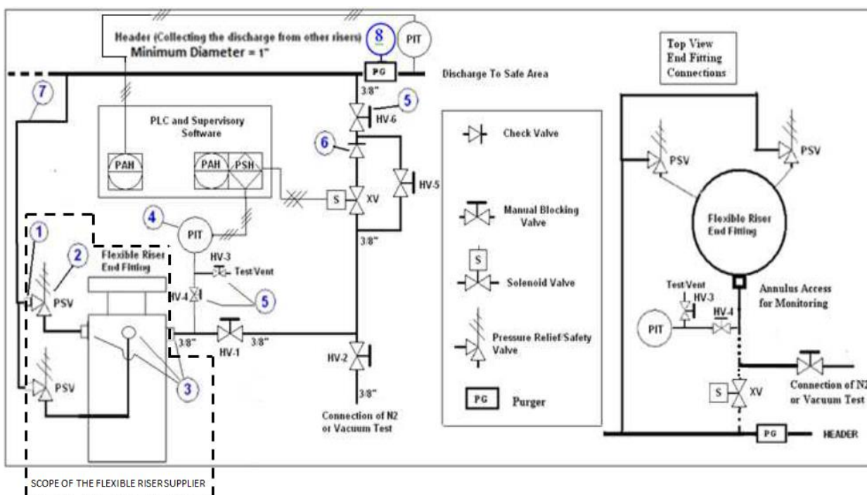
Figure 4.2 – Basic Diagram for the Automatic Type
