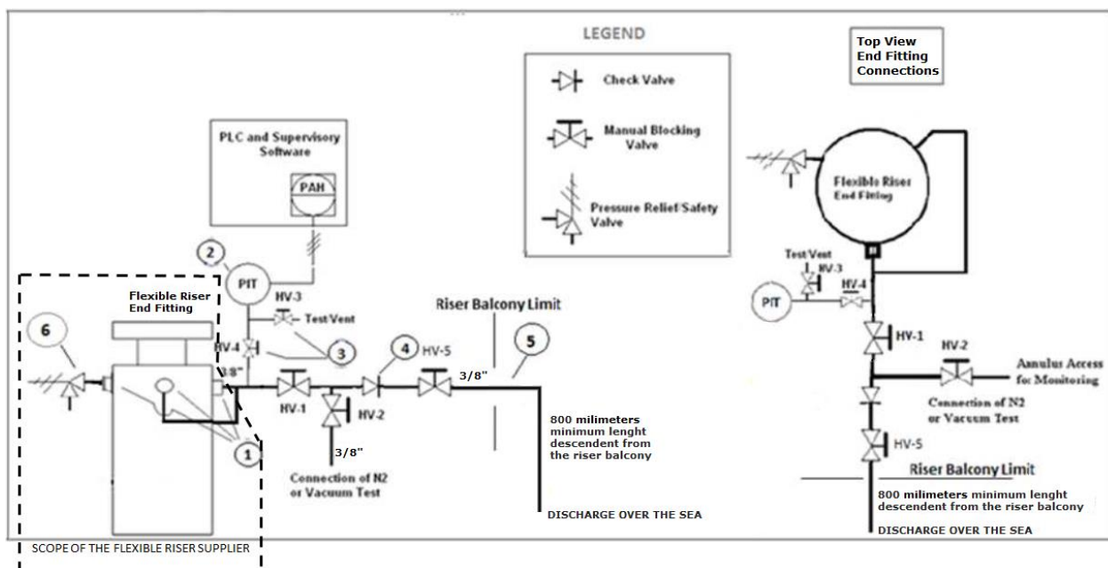
Figure 6.2 – Basic Diagram for the Local Continuous Vented Type
